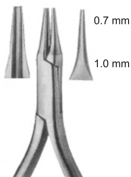
MDI-03-0031 Bending Plier 13.5cm
